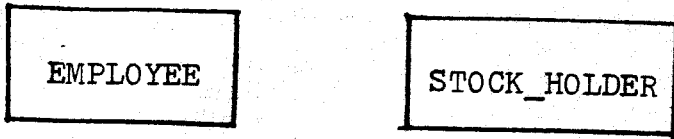
Figure 4—Entity sets
